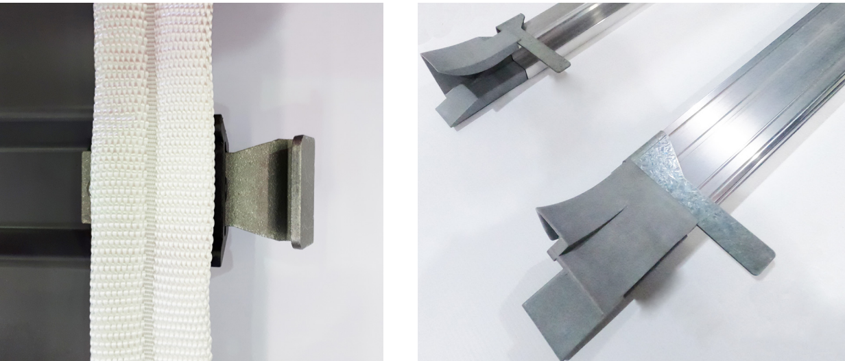
Windlock Clip
